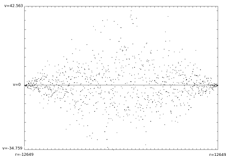
FIGURE 3. The absolute error v = \pi_{E,r}(4 \cdot 10^7) - F_{E,r}(4 \cdot 10^7)
