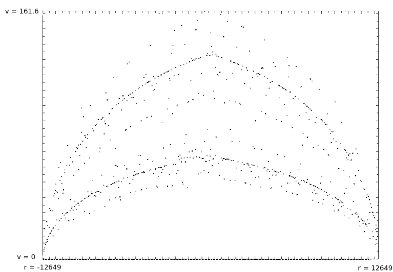
FIGURE 7. The approximation v = F_{E,r}(4 \cdot 10^7) , as a function of r
